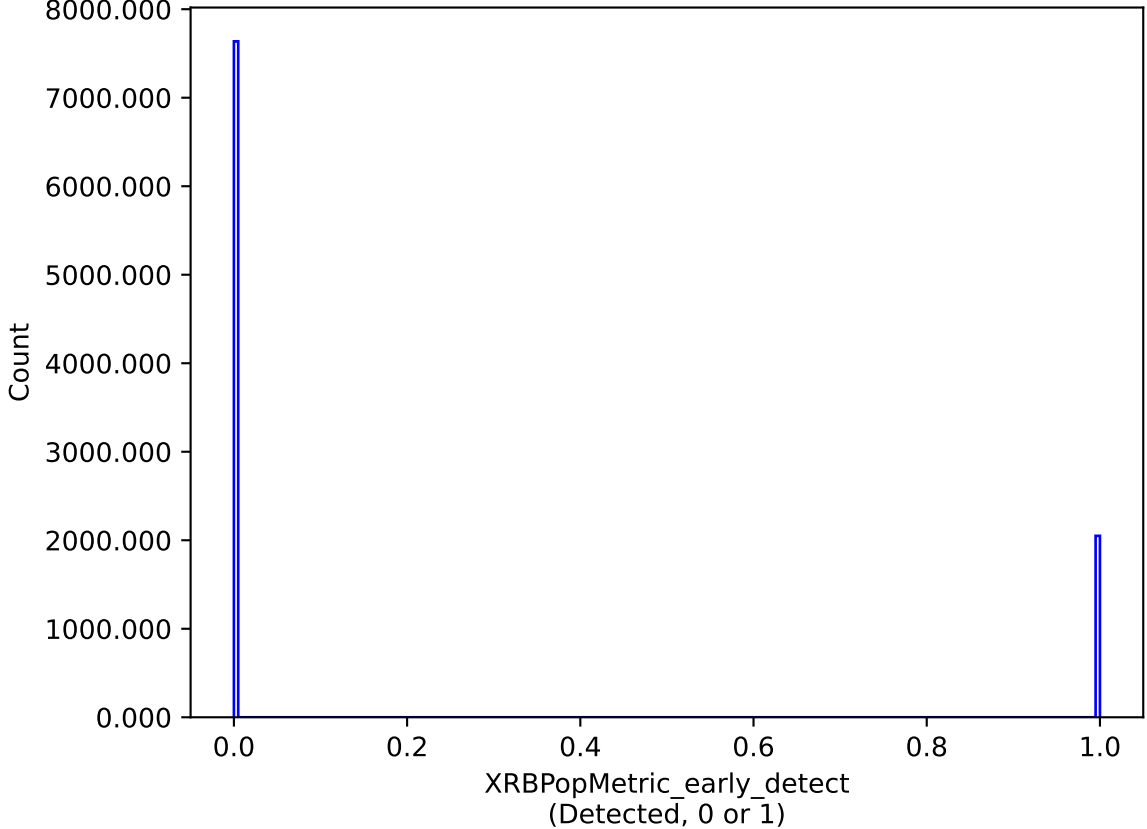
roll_pause_mjdp180_v3.4_10yrs : XRBPopMetric_early_detect
