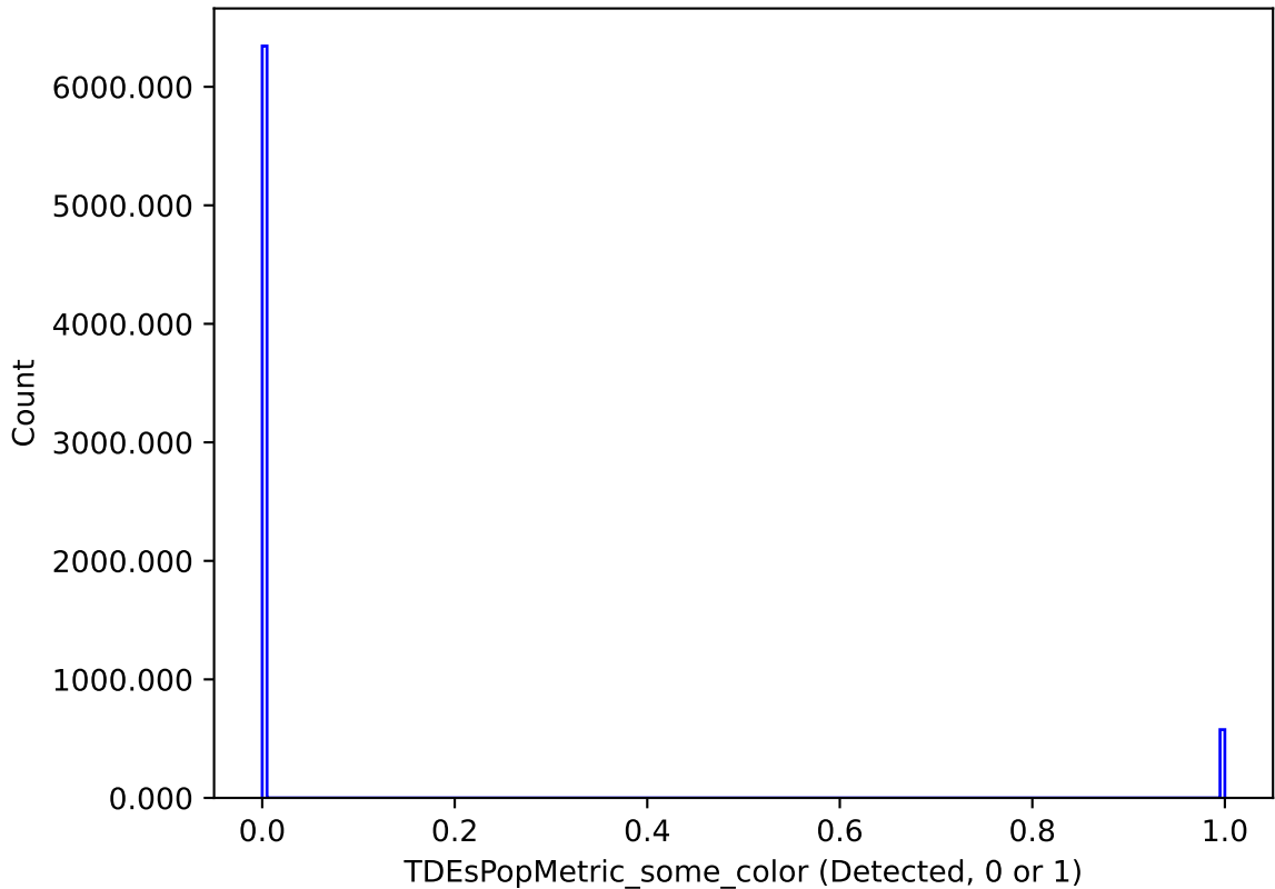
roll_pause_mjdp180_v3.4_10yrs : TDEsPopMetric_some_color
