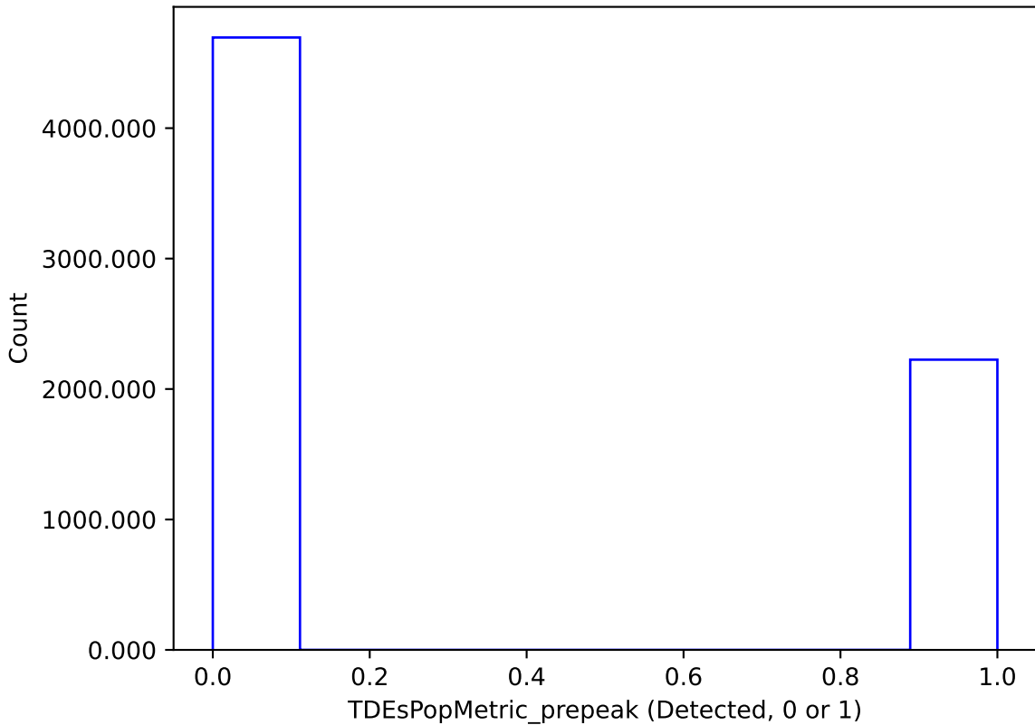
roll_pause_mjdp180_v3.4_10yrs : TDEsPopMetric_prepeak
