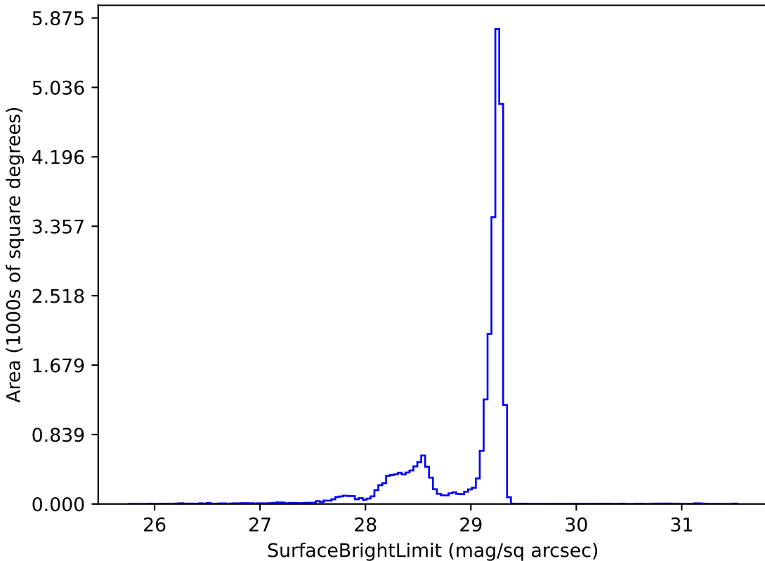
roll_pause_mjdp180_v3.4_10yrs z: SurfaceBrightLimit
