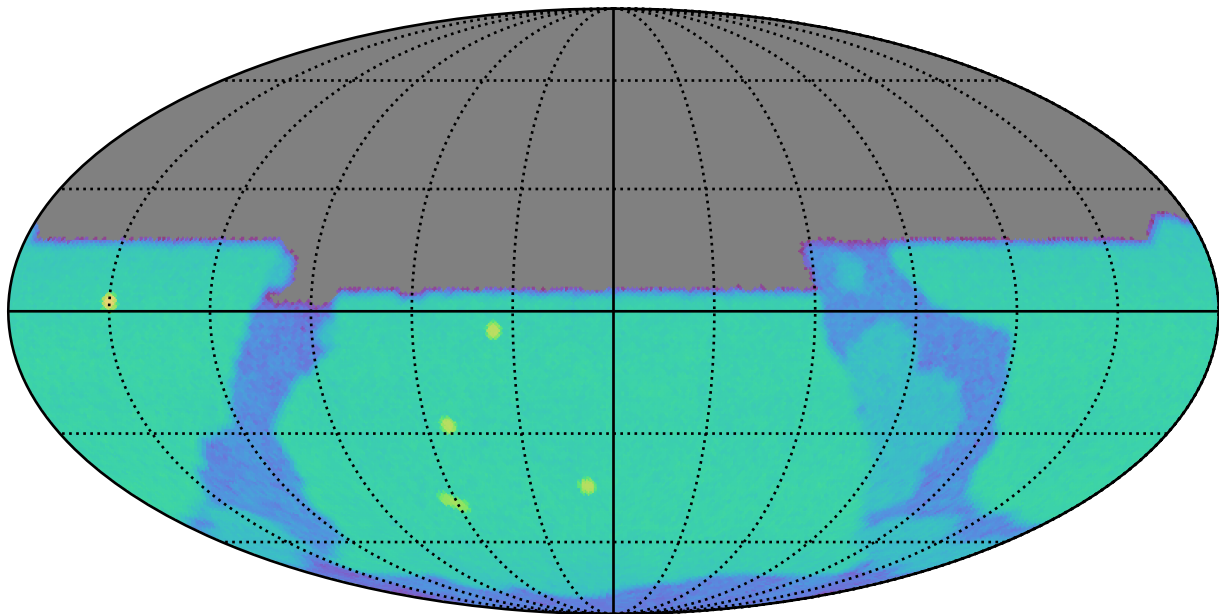
roll_pause_mjdp180_v3.4_10yrs u: SurfaceBrightLimit
