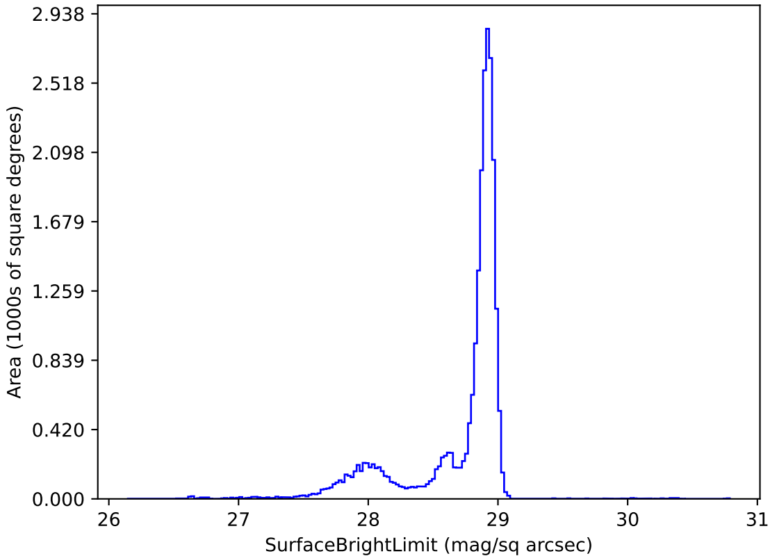
roll_pause_mjdp180_v3.4_10yrs u: SurfaceBrightLimit
