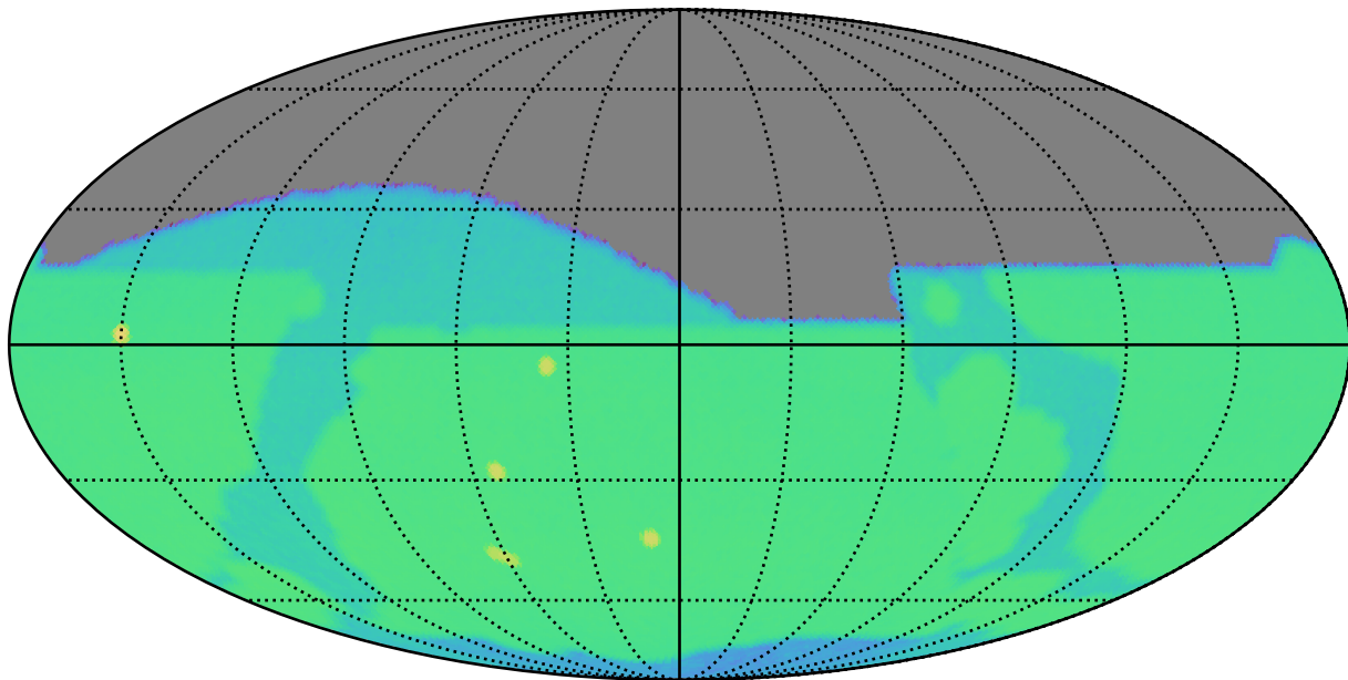
roll_pause_mjdp180_v3.4_10yrs r: SurfaceBrightLimit
