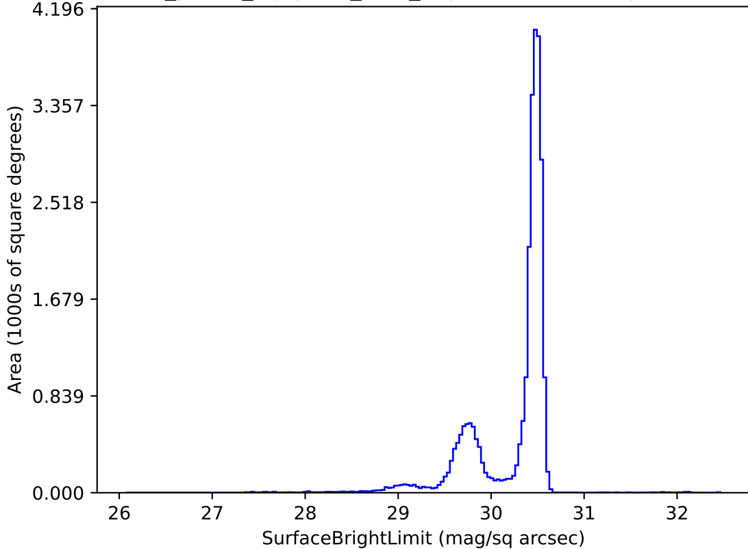
roll_pause_mjdp180_v3.4_10yrs r: SurfaceBrightLimit
