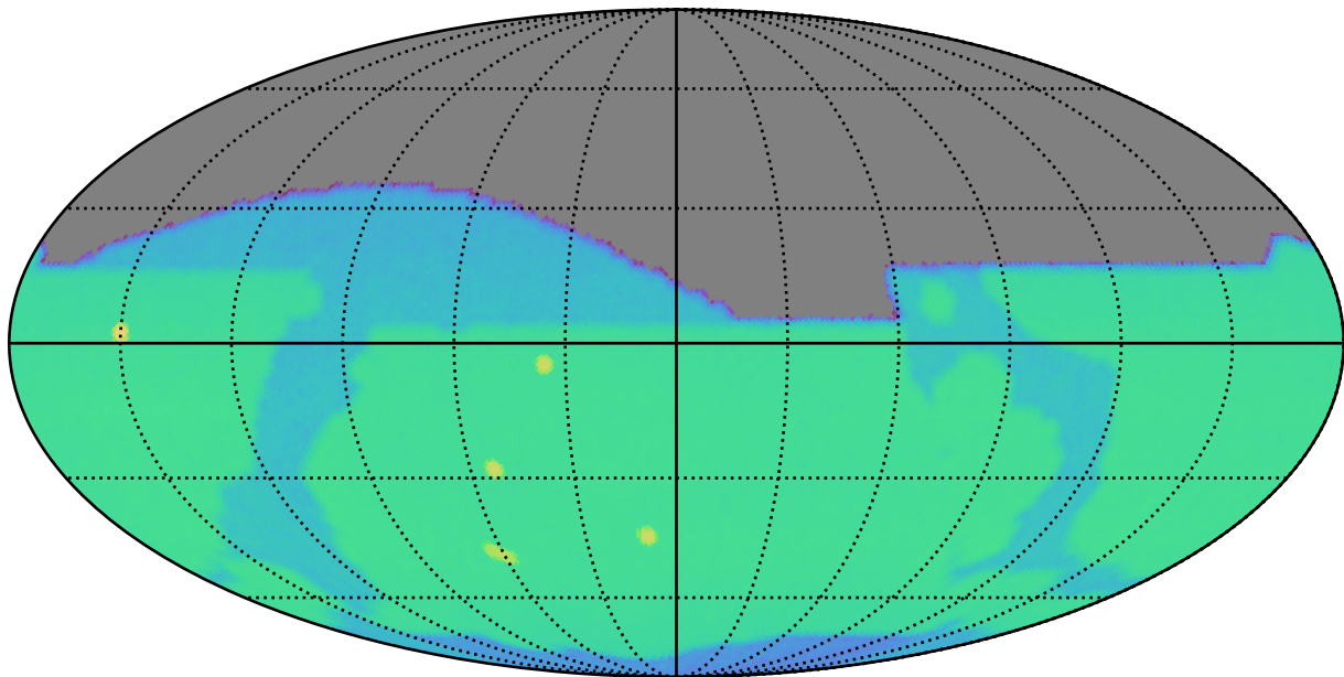
roll_pause_mjdp180_v3.4_10yrs i: SurfaceBrightLimit
