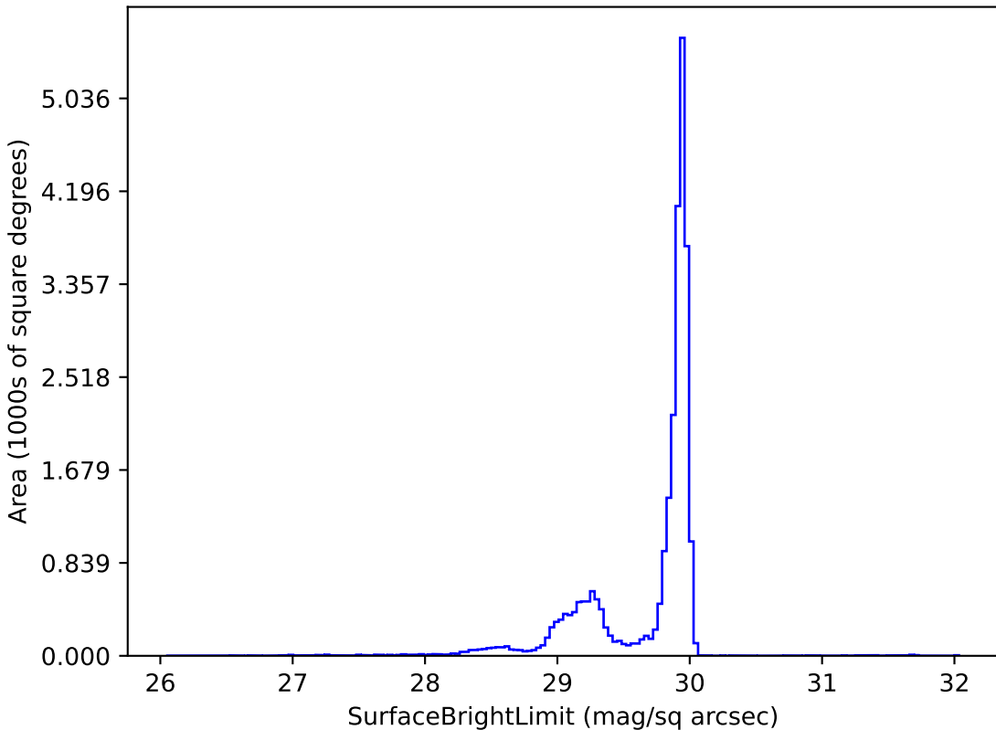
roll_pause_mjdp180_v3.4_10yrs i: SurfaceBrightLimit
