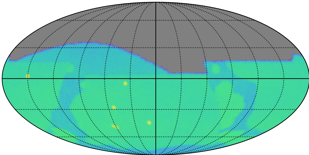
roll_pause_mjdp180_v3.4_10yrs g: SurfaceBrightLimit
