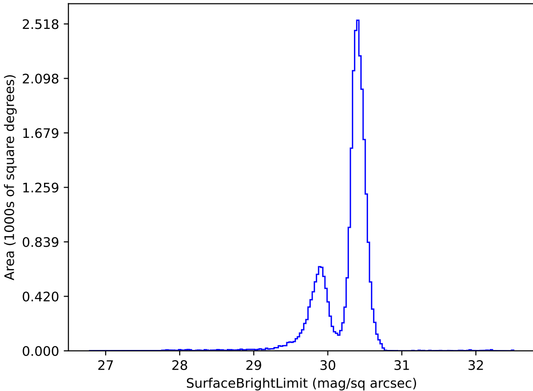
roll_pause_mjdp180_v3.4_10yrs g: SurfaceBrightLimit
