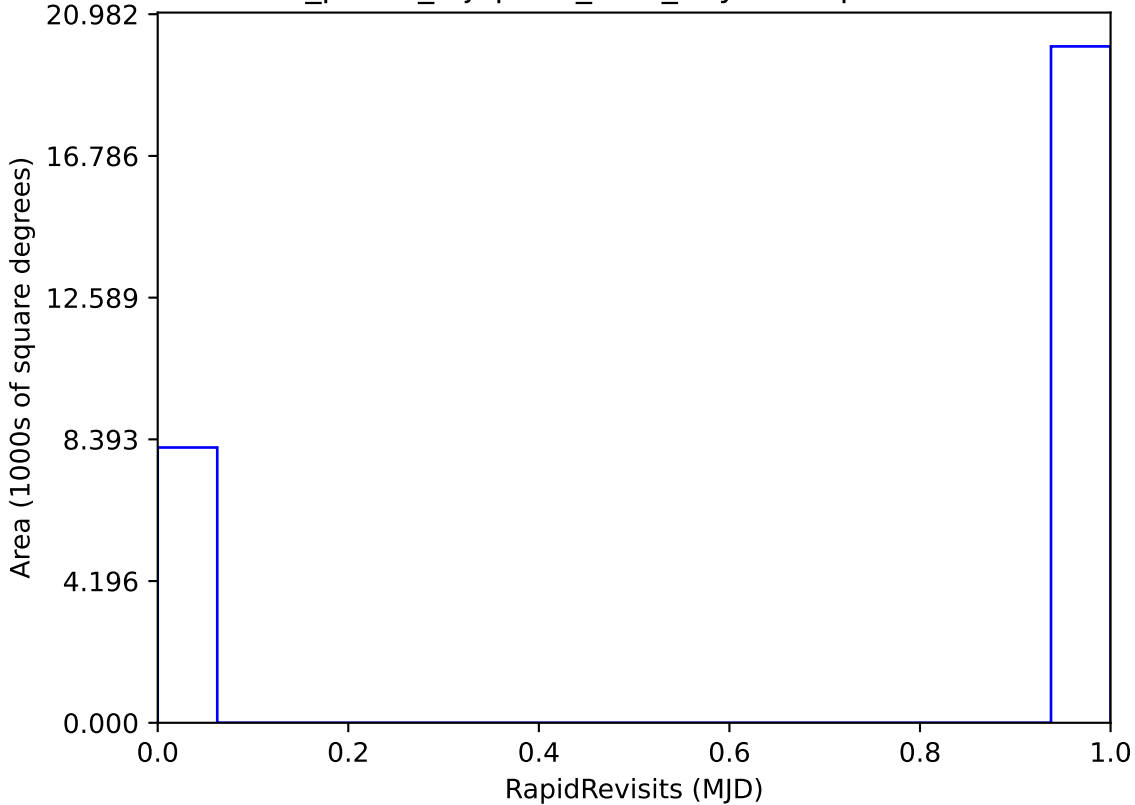
roll_pause_mjdp180_v3.4_10yrs : RapidRevisits
