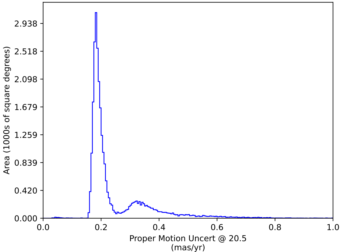
roll_pause_mjdp180_v3.4_10yrs : Proper Motion Uncert @ 20.5
