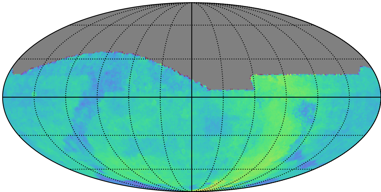
roll_pause_mjdp180_v3.4_10yrs : Parallax Coverage @ 24.0
