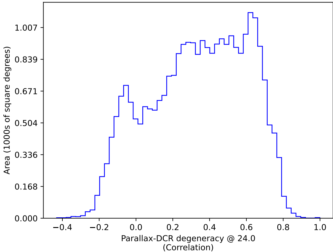
roll_pause_mjdp180_v3.4_10yrs : Parallax-DCR degeneracy @ 24.0
