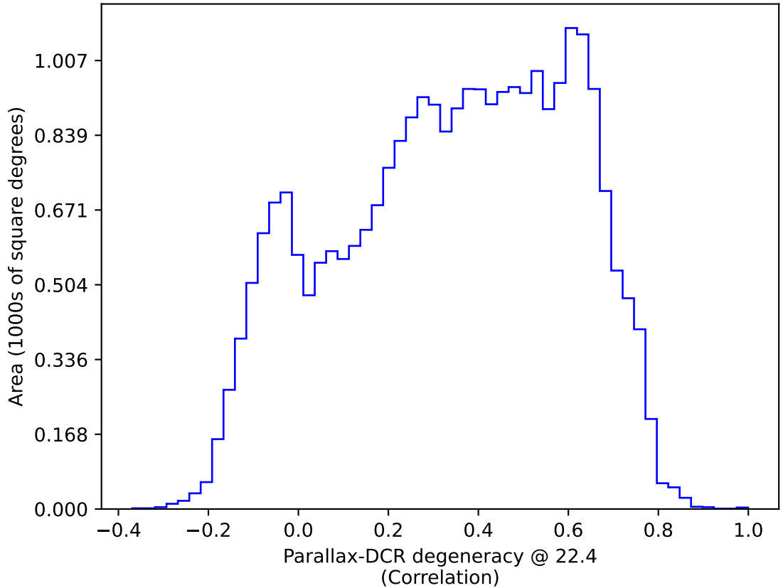
roll_pause_mjdp180_v3.4_10yrs : Parallax-DCR degeneracy @ 22.4
