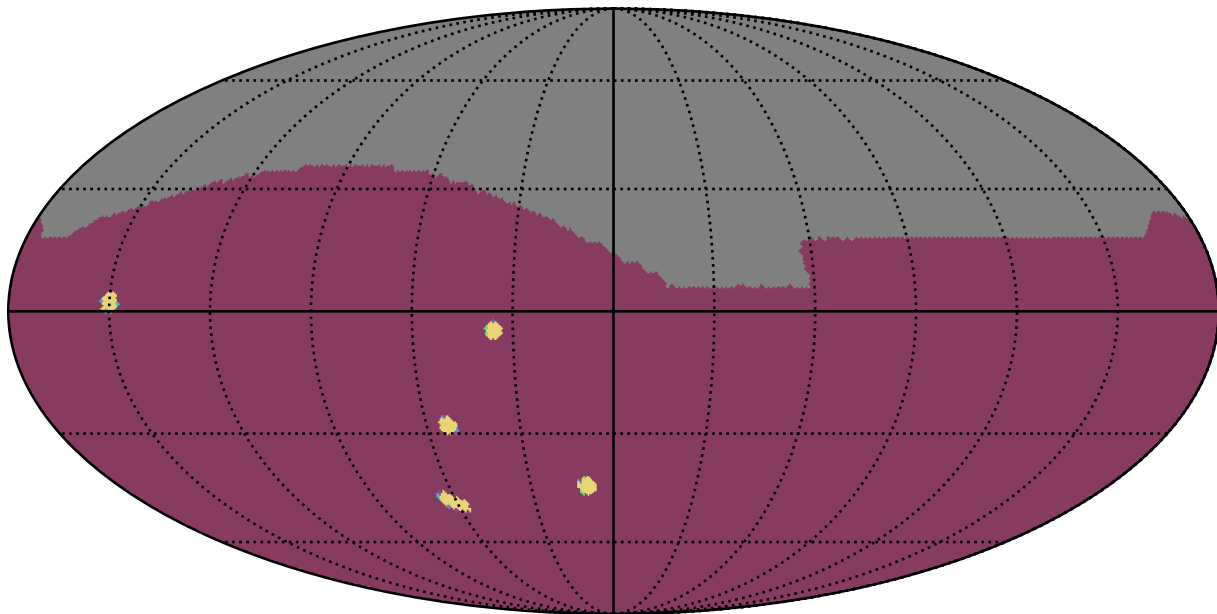
roll_pause_mjdp180_v3.4_10yrs : NumberOfQuickRevisits
