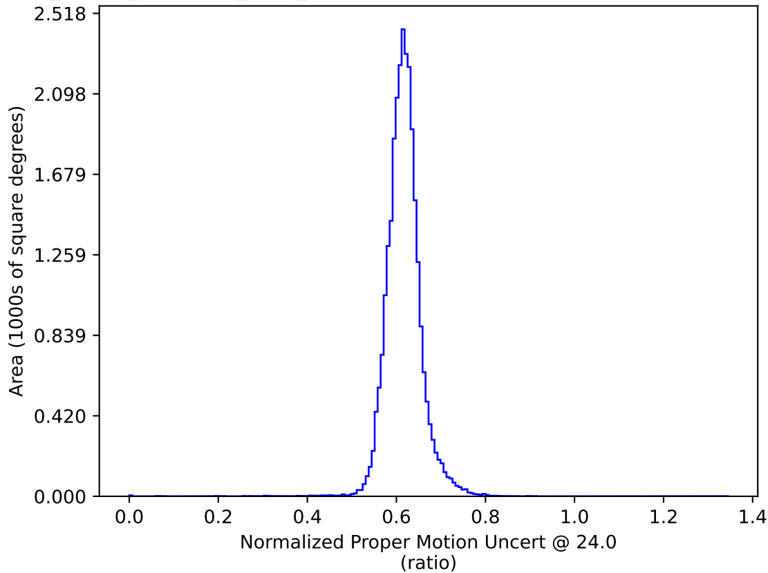
roll_pause_mjdp180_v3.4_10yrs : Normalized Proper Motion Uncert @ 24.0
