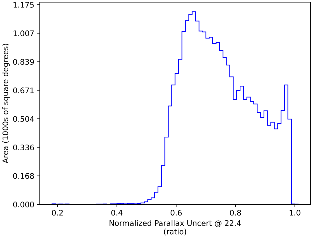
roll_pause_mjdp180_v3.4_10yrs : Normalized Parallax Uncert @ 22.4
