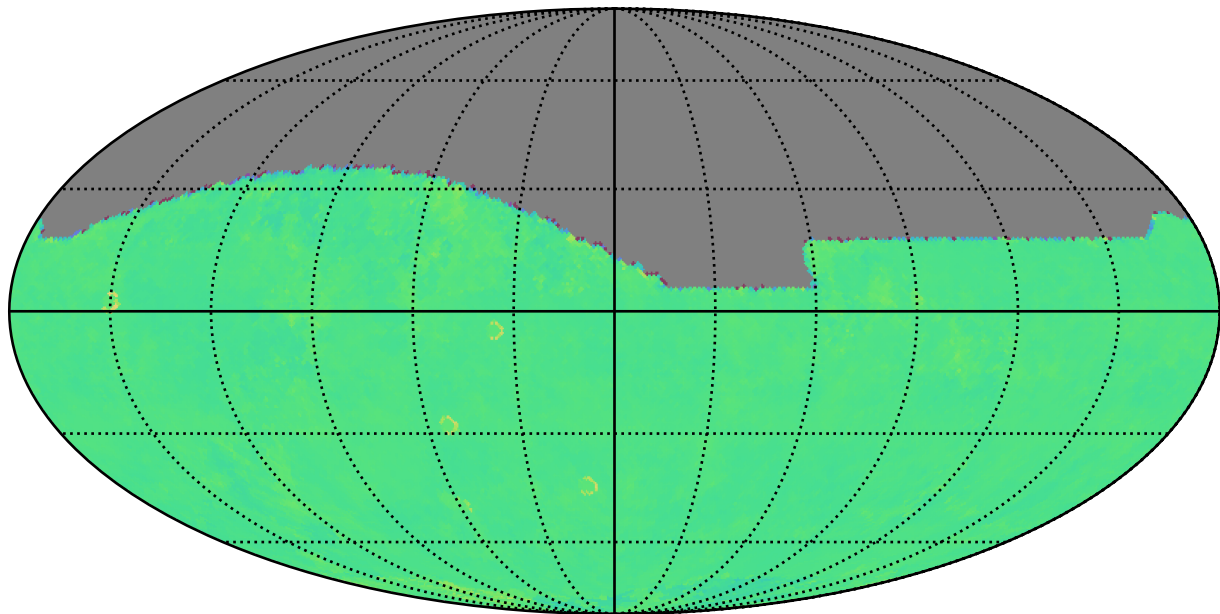
roll_pause_mjdp180_v3.4_10yrs z: Kuiper rotTelPos
