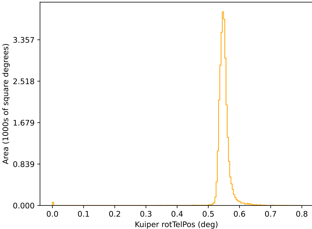
roll_pause_mjdp180_v3.4_10yrs r: Kuiper rotTelPos
