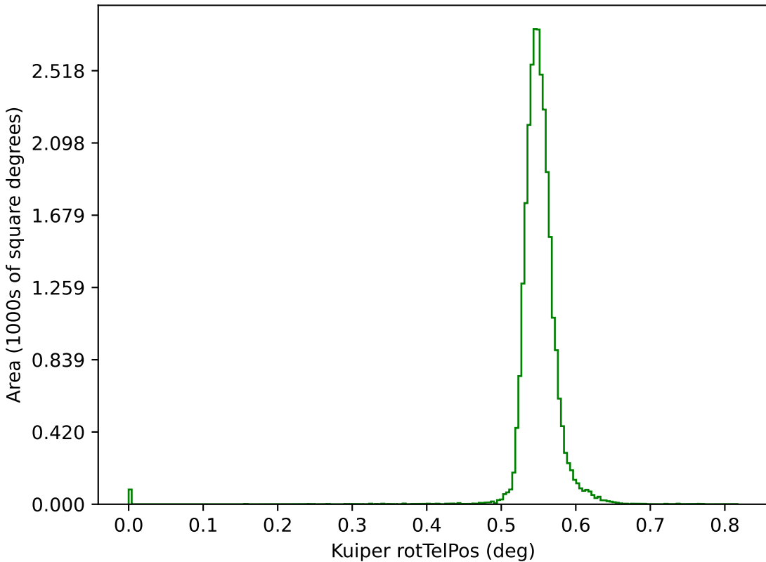
roll_pause_mjdp180_v3.4_10yrs g: Kuiper rotTelPos
