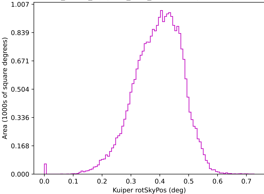
roll_pause_mjdp180_v3.4_10yrs z: Kuiper rotSkyPos
