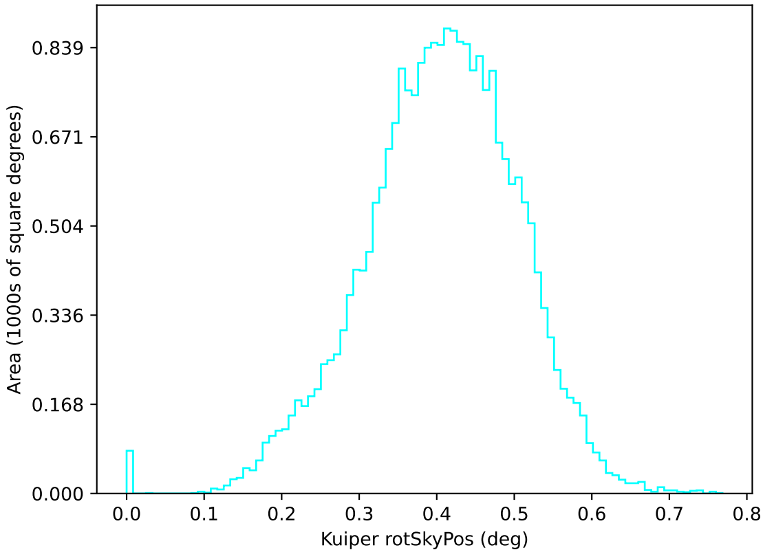
roll_pause_mjdp180_v3.4_10yrs u: Kuiper rotSkyPos
