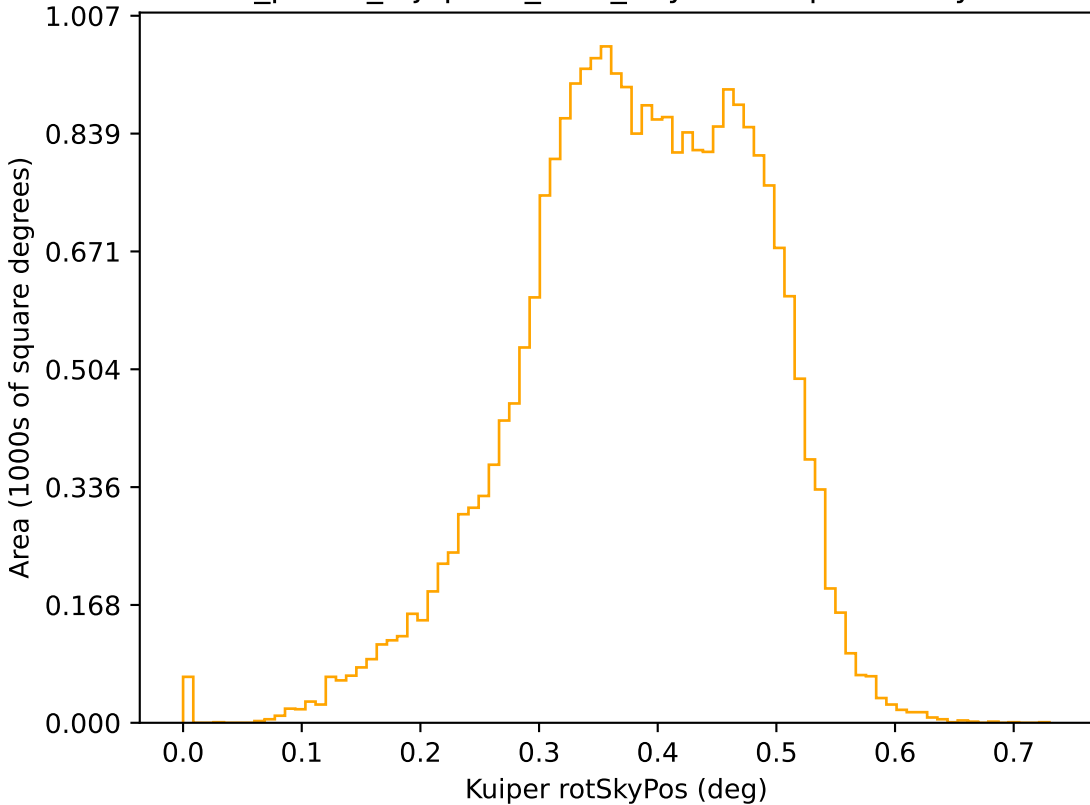
roll_pause_mjdp180_v3.4_10yrs r: Kuiper rotSkyPos
