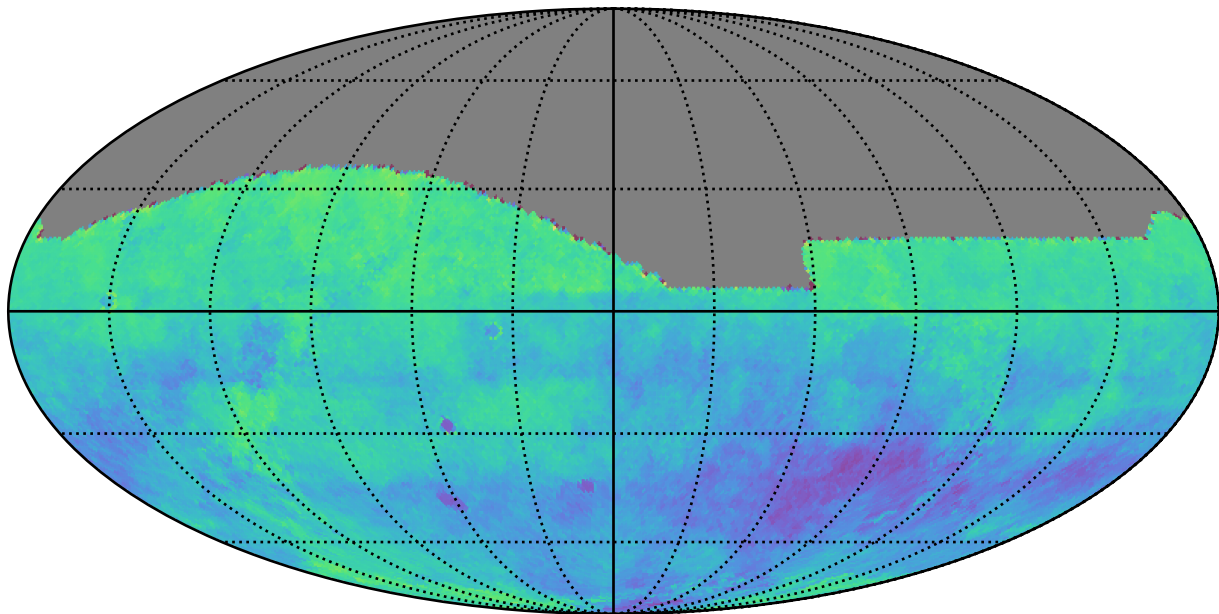
roll_pause_mjdp180_v3.4_10yrs i: Kuiper rotSkyPos
