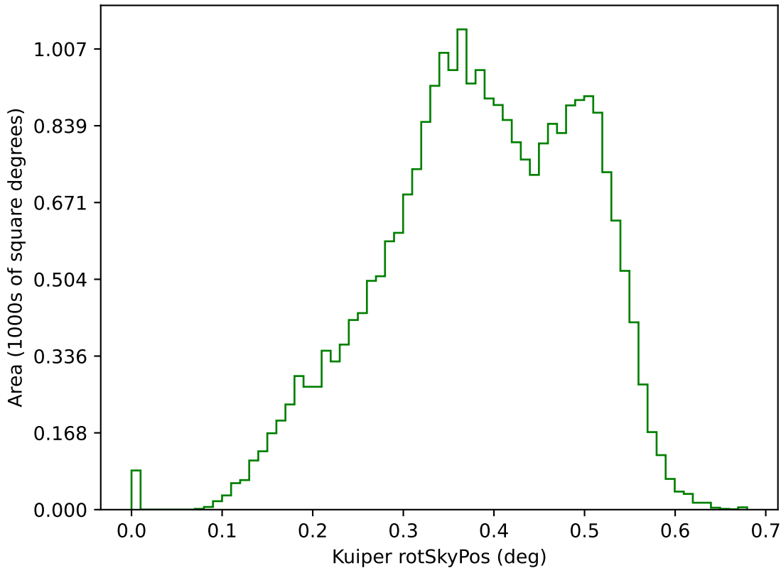
roll_pause_mjdp180_v3.4_10yrs g: Kuiper rotSkyPos
