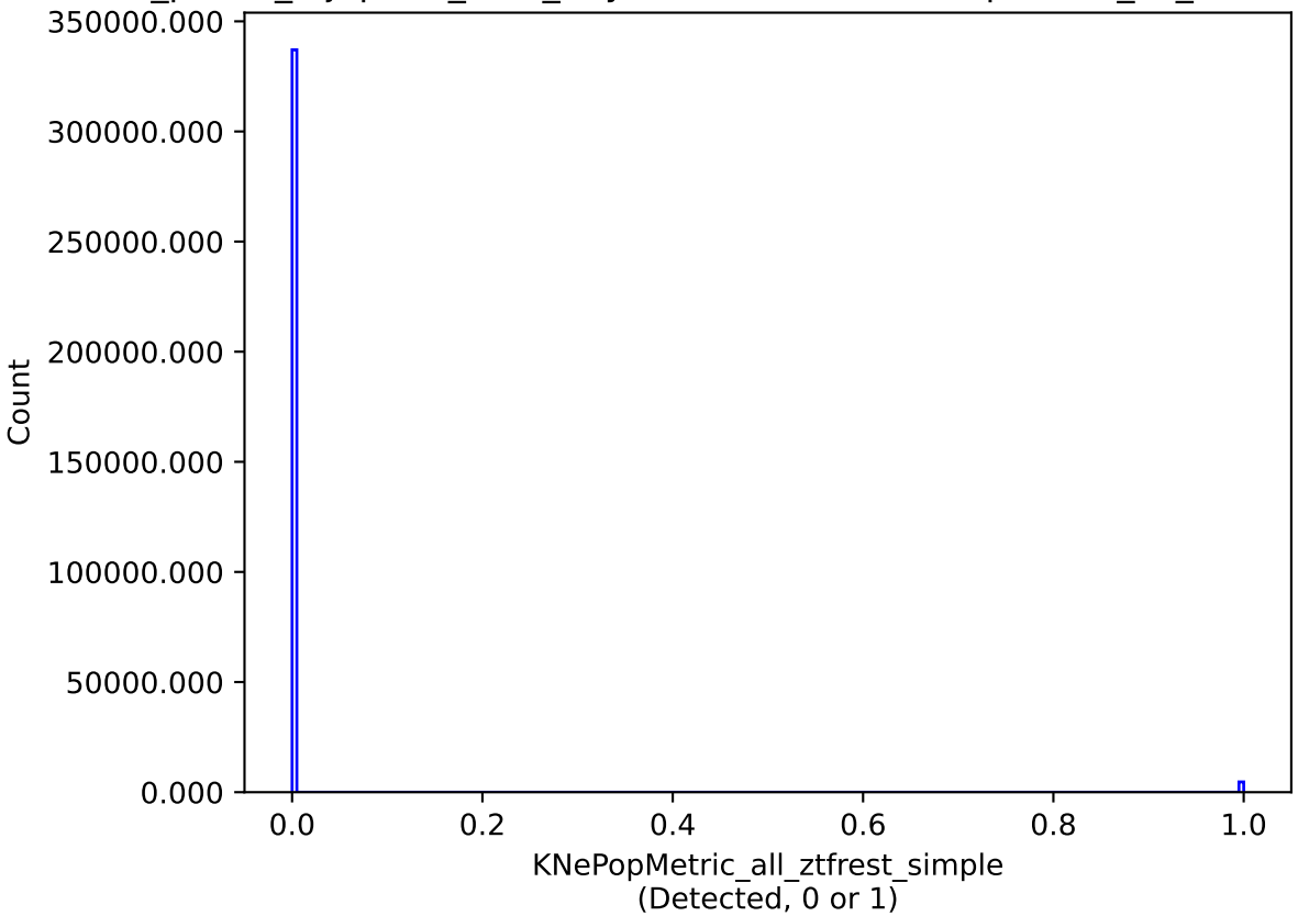
roll_pause_mjdp180_v3.4_10yrs all models: KNePopMetric_all_ztfrest_simple
