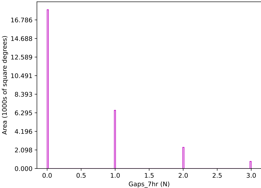
roll_pause_mjdp180_v3.4_10yrs z band: Gaps_7hr
