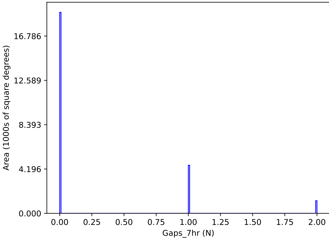
roll_pause_mjdp180_v3.4_10yrs y band: Gaps_7hr
