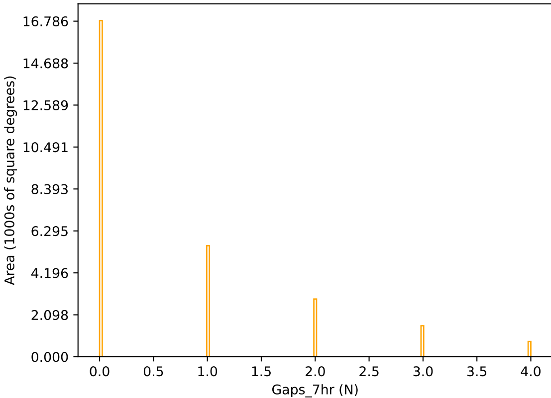
roll_pause_mjdp180_v3.4_10yrs r band: Gaps_7hr
