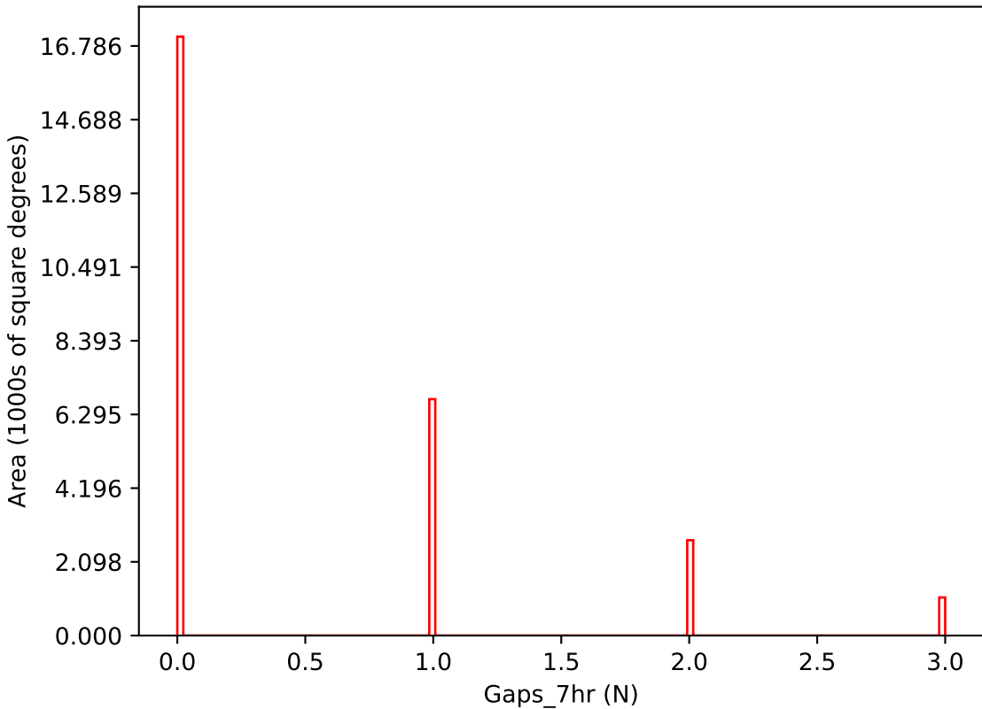
roll_pause_mjdp180_v3.4_10yrs i band: Gaps_7hr
