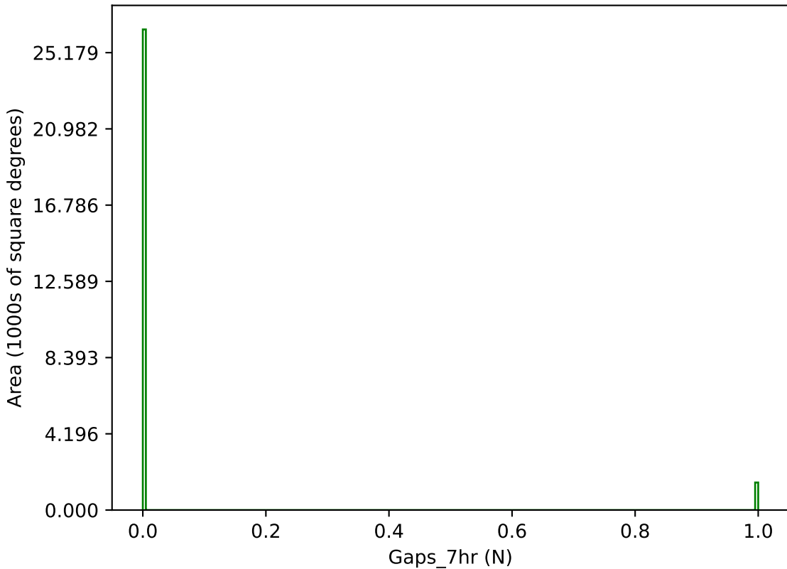
roll_pause_mjdp180_v3.4_10yrs g band: Gaps_7hr
