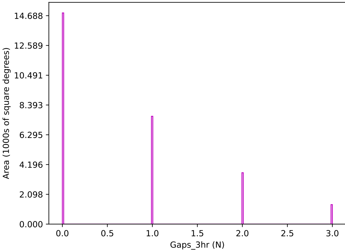
roll_pause_mjdp180_v3.4_10yrs z band: Gaps_3hr
