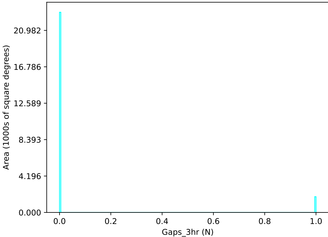
roll_pause_mjdp180_v3.4_10yrs u band: Gaps_3hr
