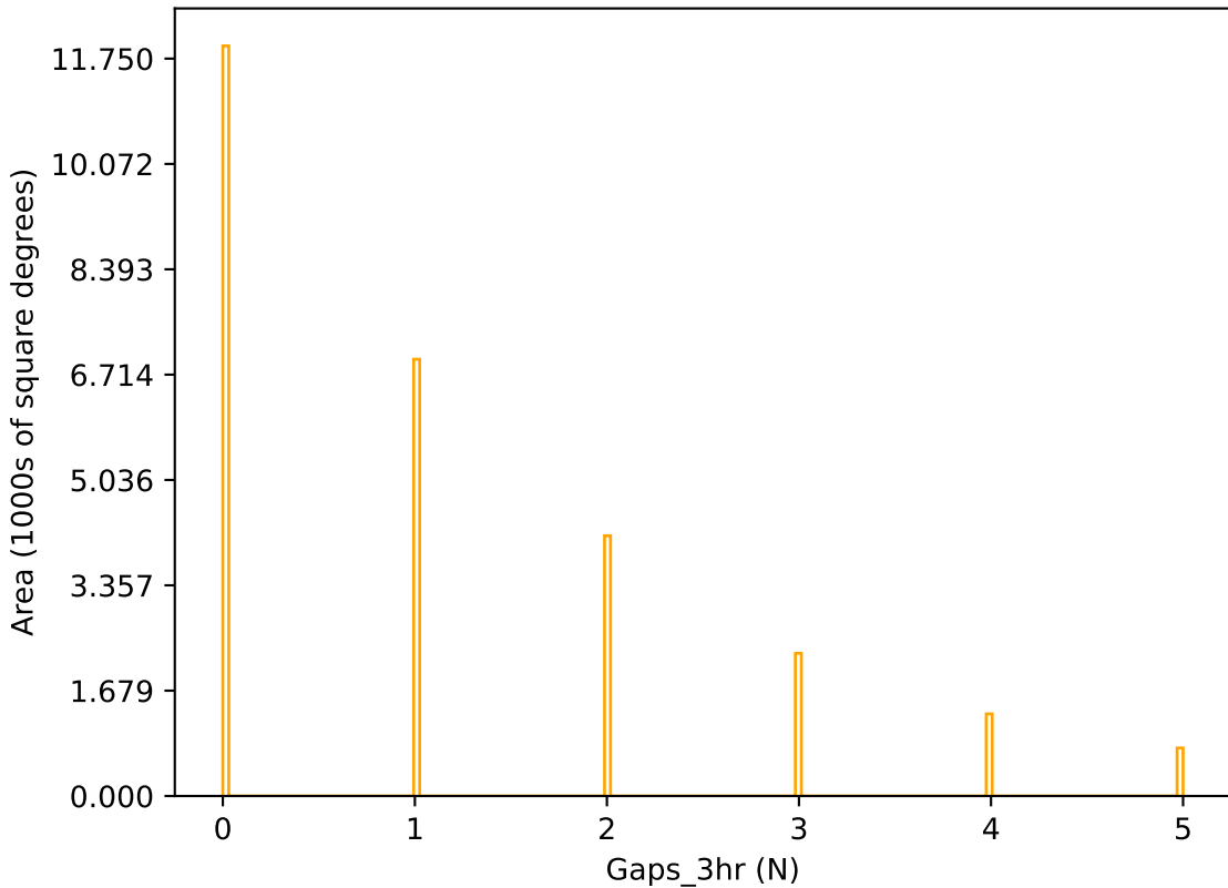
roll_pause_mjdp180_v3.4_10yrs r band: Gaps_3hr
