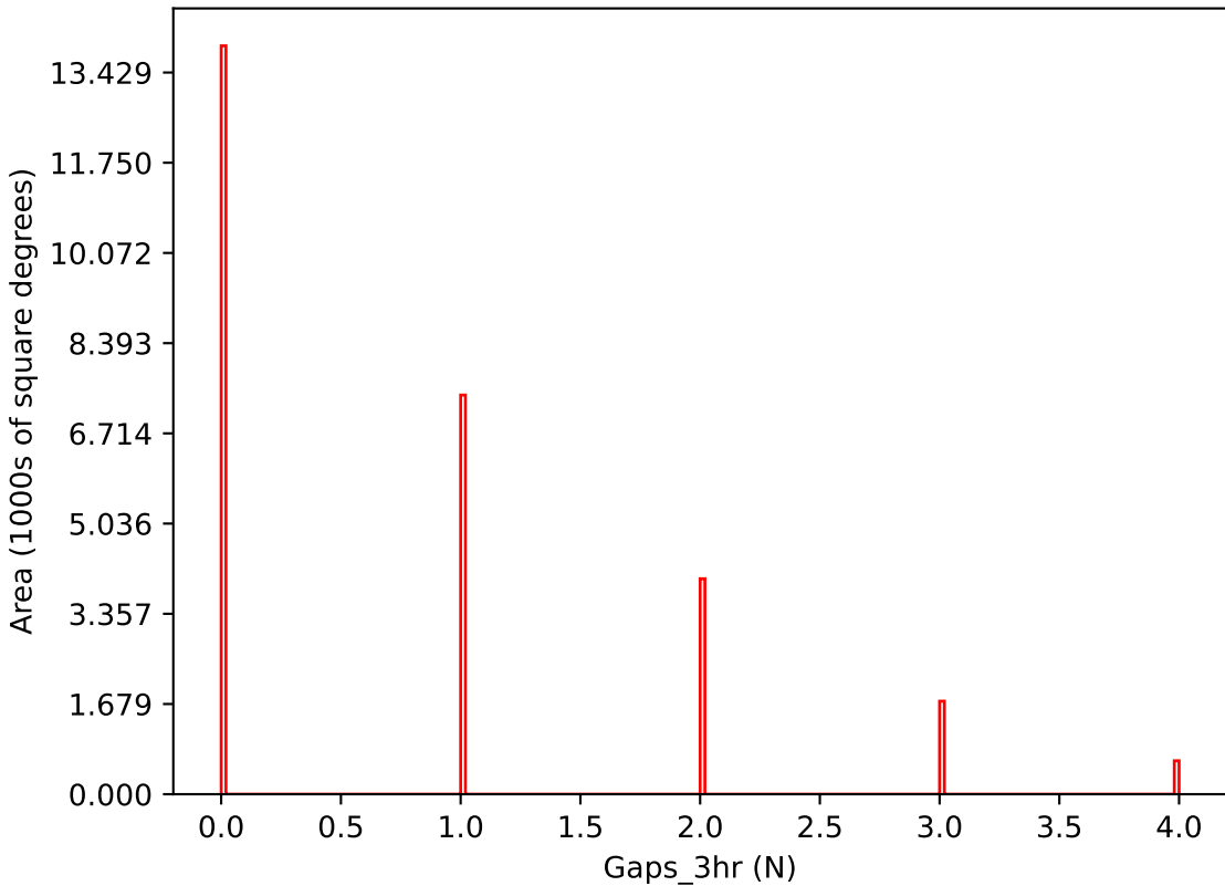
roll_pause_mjdp180_v3.4_10yrs i band: Gaps_3hr
