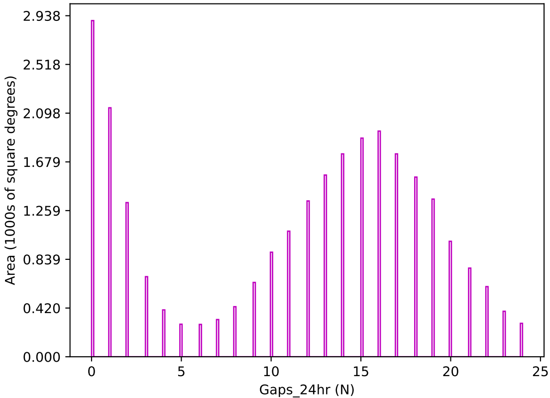
roll_pause_mjdp180_v3.4_10yrs z band: Gaps_24hr
