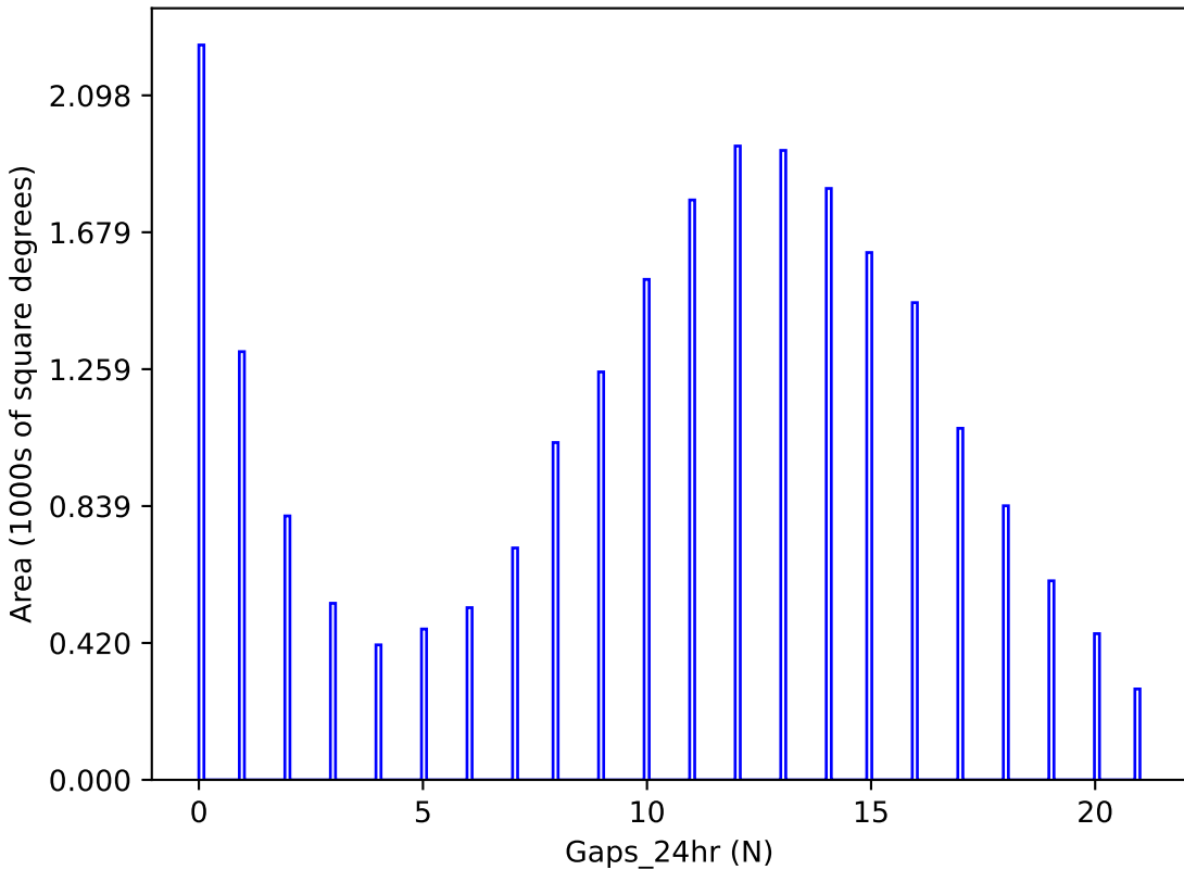
roll_pause_mjdp180_v3.4_10yrs y band: Gaps_24hr
