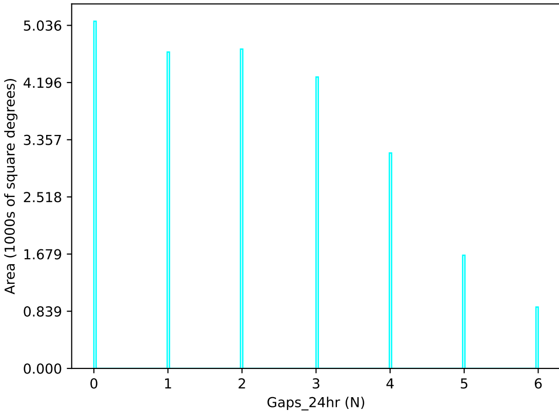
roll_pause_mjdp180_v3.4_10yrs u band: Gaps_24hr
