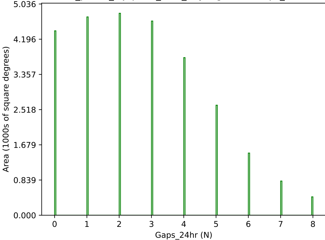
roll_pause_mjdp180_v3.4_10yrs g band: Gaps_24hr
