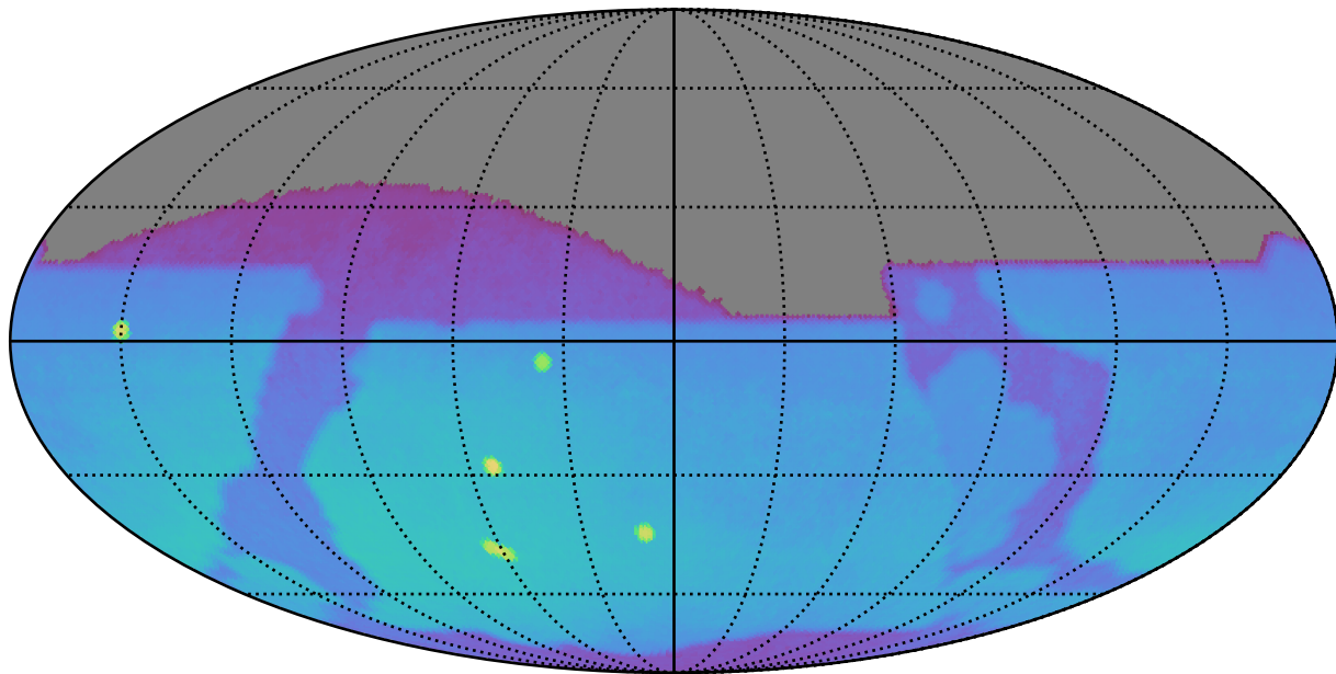
roll_pause_mjdp180_v3.4_10yrs : Brown Dwarf, L7
