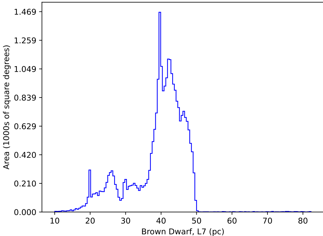
roll_pause_mjdp180_v3.4_10yrs : Brown Dwarf, L7
