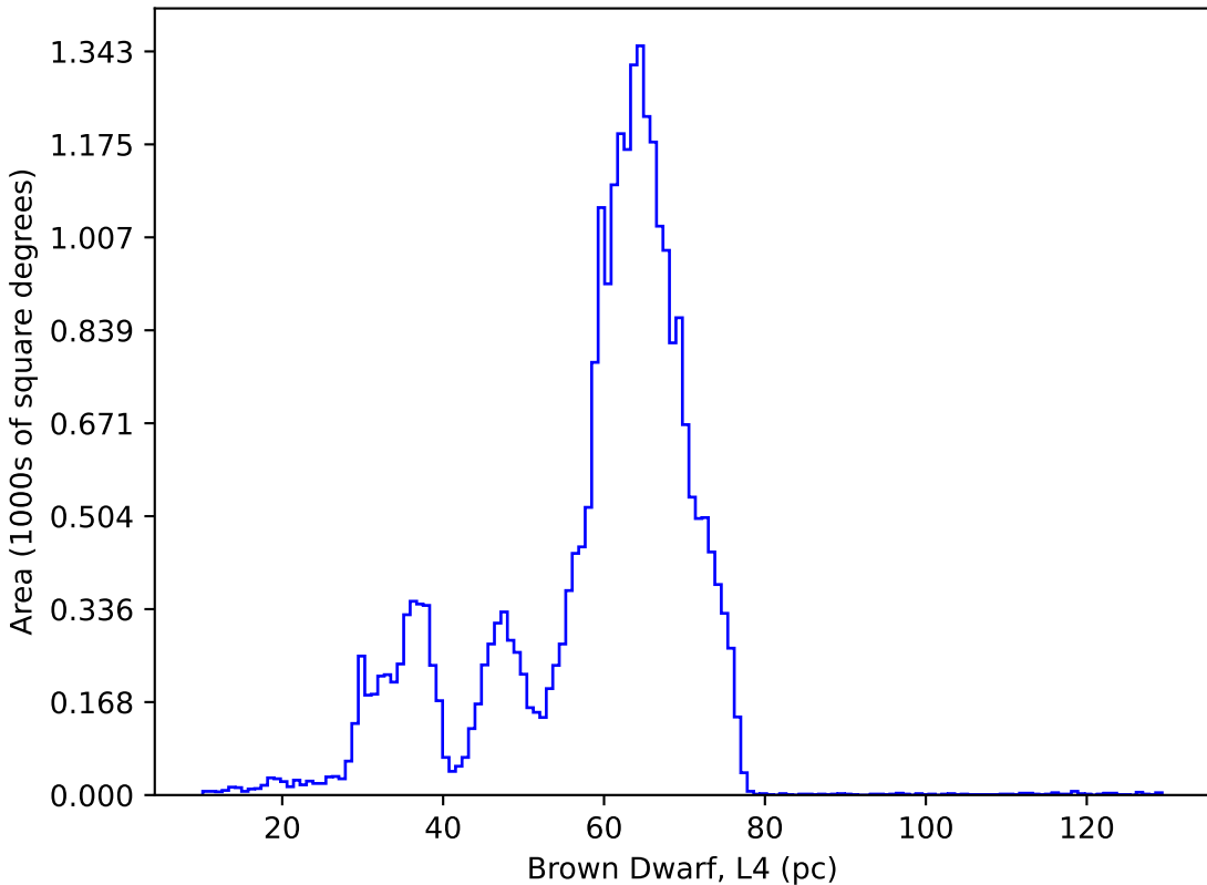
roll_pause_mjdp180_v3.4_10yrs : Brown Dwarf, L4
