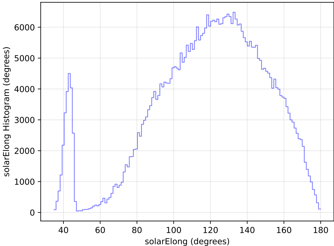
roll_pause_mjdp180_v3.4_10yrs WFD z band: solarElong Histogram
