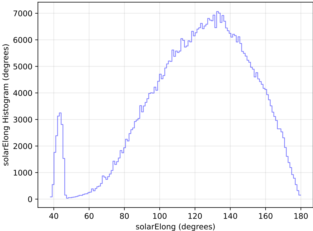
roll_pause_mjdp180_v3.4_10yrs WFD r band: solarElong Histogram
