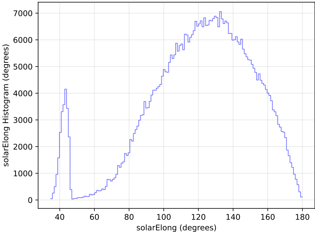
roll_pause_mjdp180_v3.4_10yrs WFD i band: solarElong Histogram
