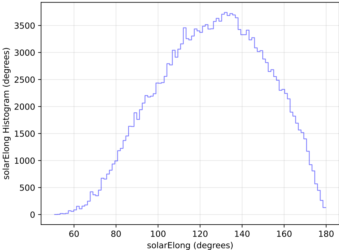
roll_pause_mjdp180_v3.4_10yrs WFD g band: solarElong Histogram
