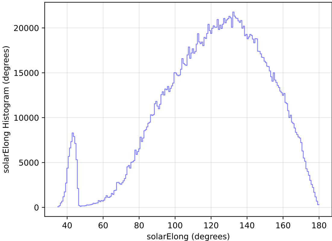
roll_pause_mjdp180_v3.4_10yrs WFD all bands: solarElong Histogram
